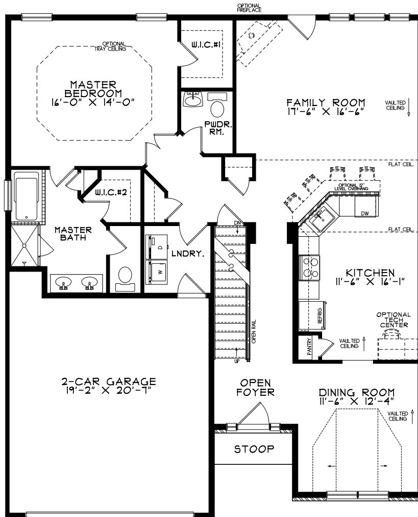
OLYMPIA FIRST FLOOR PLAN 1,420sf
