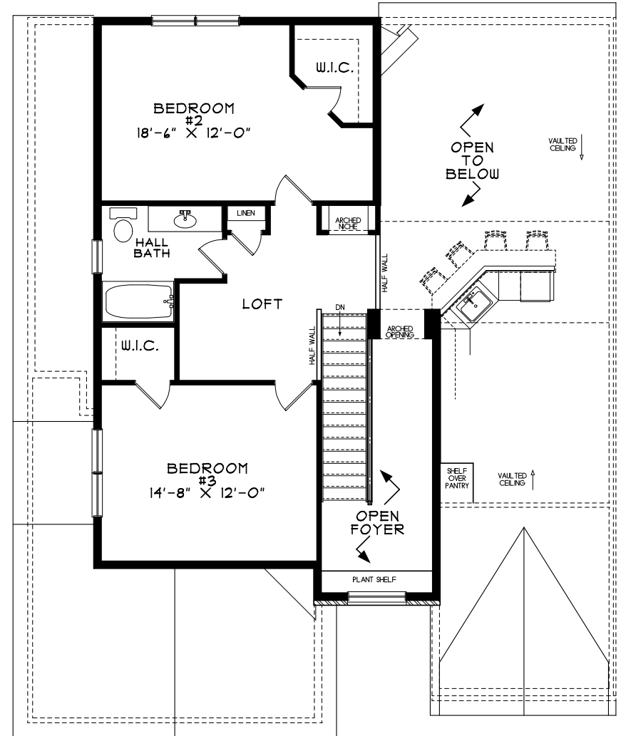
OLYMPIA SECOND FLOOR PLAN 706sf
