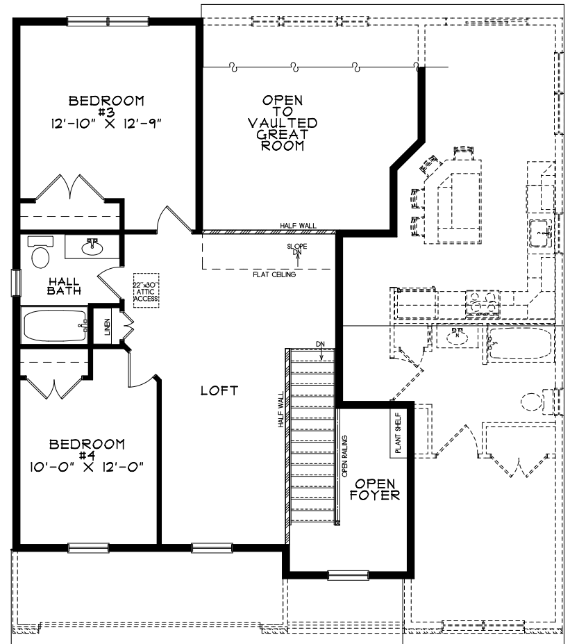
BEAUMONT II SECOND FLOOR PLAN 768sf
