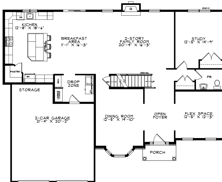
MONTCLAIR GRANDE FIRST FLOOR PLAN 1,729sf
