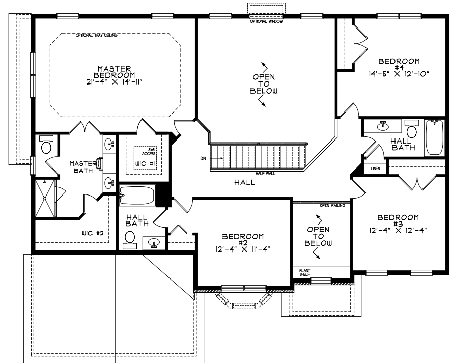
MONTCLAIR GRANDE SECOND FLOOR PLAN 1,519sf
