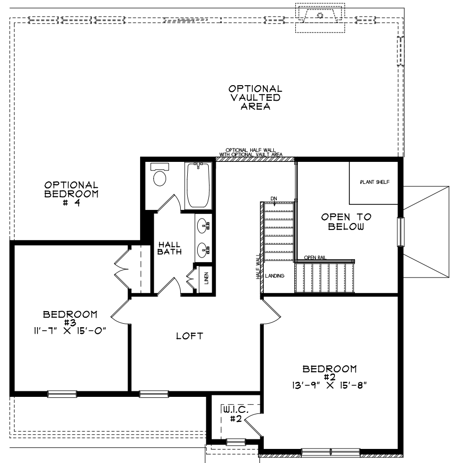
FOLCROFT SECOND FLOOR PLAN 855sf
