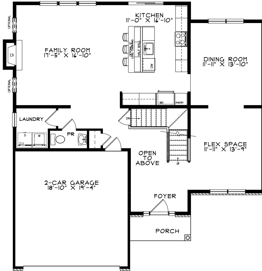
BRYCE FIRST FLOOR PLAN 1,219sf
