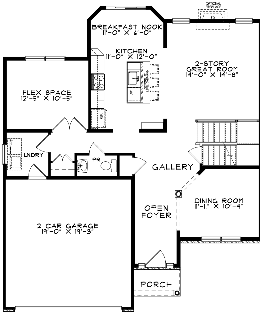
GOSSAMER FIRST FLOOR PLAN 1,105sf
