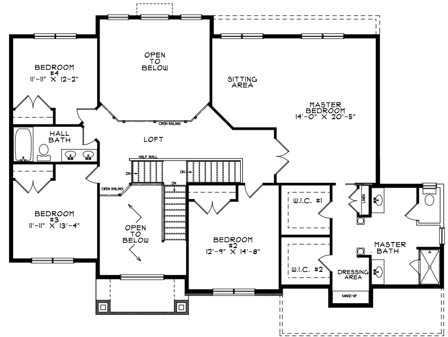
WHITMORE SECOND FLOOR PLAN 1664sf
