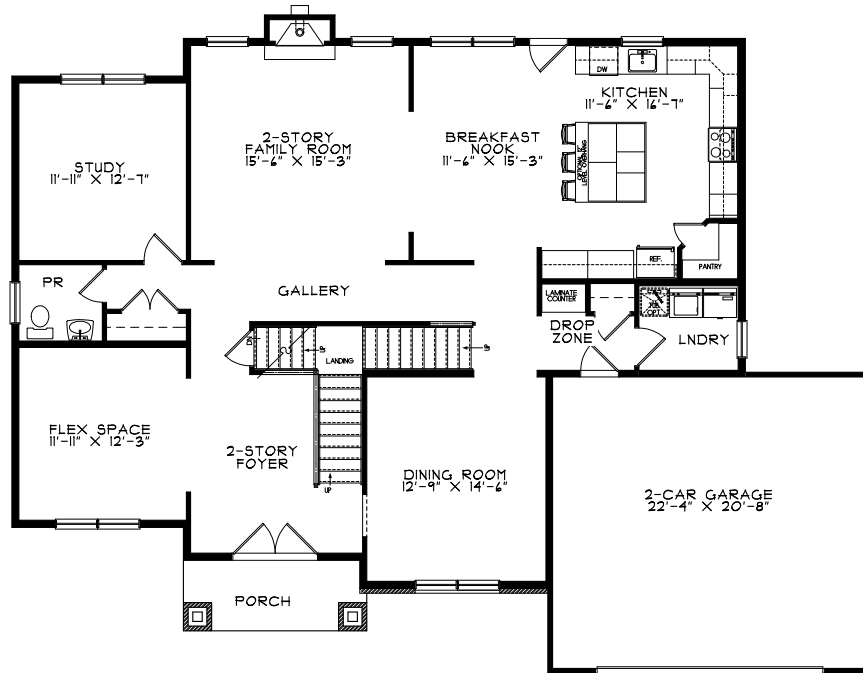
WHITMORE FIRST FLOOR PLAN 1655sf
