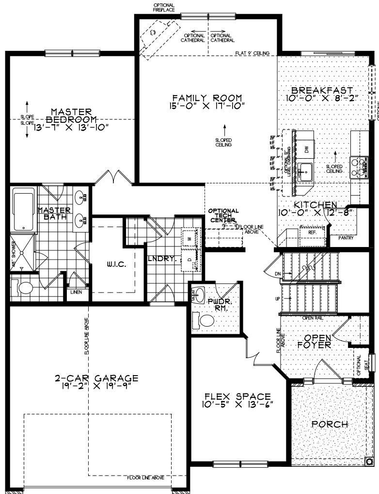
DAGGERWING FIRST FLOOR PLAN 1441sf
