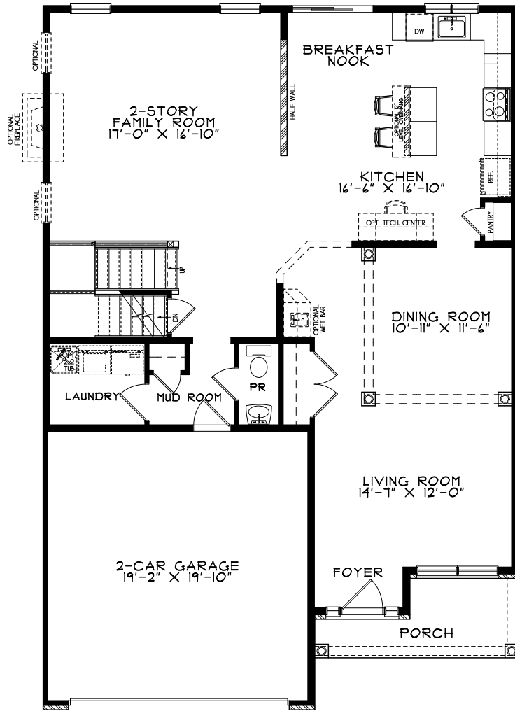
MONARCH FIRST FLOOR PLAN 1,284sf
