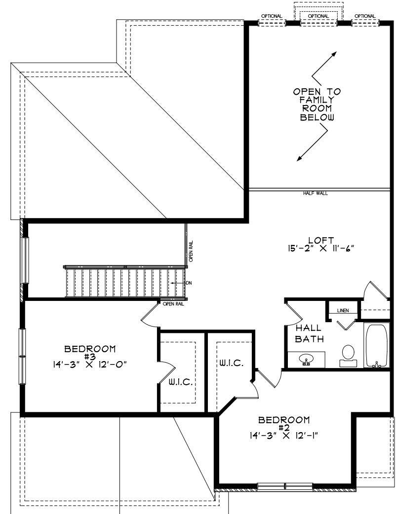
LUNA SECOND FLOOR PLAN 919sf
