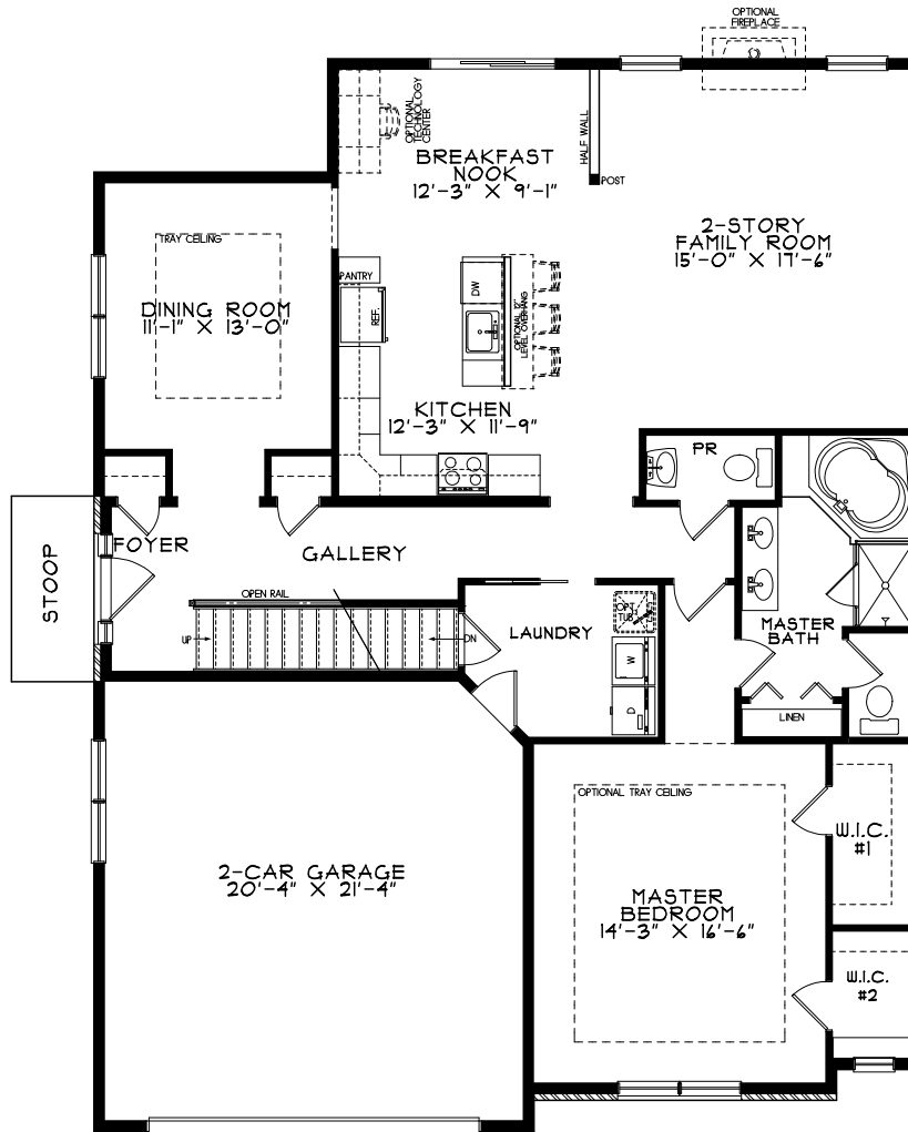
LUNA FIRST FLOOR PLAN 1,533sf
