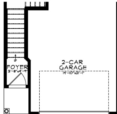
OPTIONAL TERRACE LEVEL PLAN
